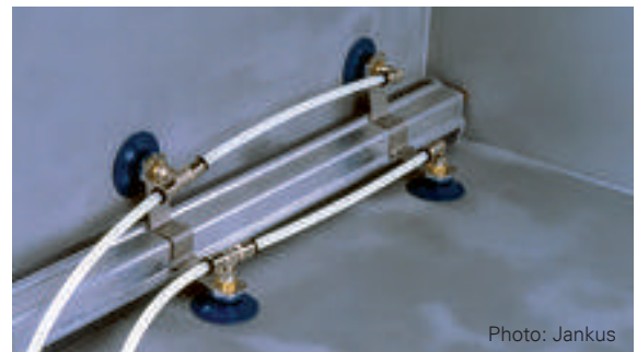
Shield gas angle profile for corner seams
